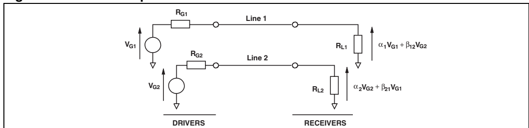
Figure 14. Crosstalk phenomena
